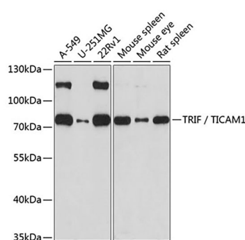
Fig. 1. Western blot analysis of extracts of various cell lines, using TRIF / TICAM1 antibody at 1:1000 dilution. Secondary antibody: HRP-labeled Goat Anti-Rabbit IgG(H+L) (A0208) at 1:1000 dilution. Lysates/proteins: 25 \mu g per lane. Blocking buffer: QuickBlock TM Blocking Buffer (P0231). Detection: BeyoECL Star (P0018A). Exposure time: 1s.
